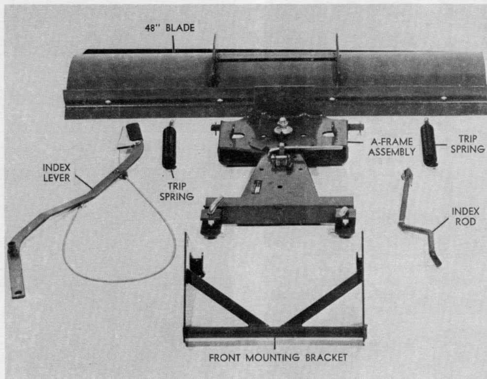
FIG. 1. 48" Snow/Dozer Blade 6-0700
